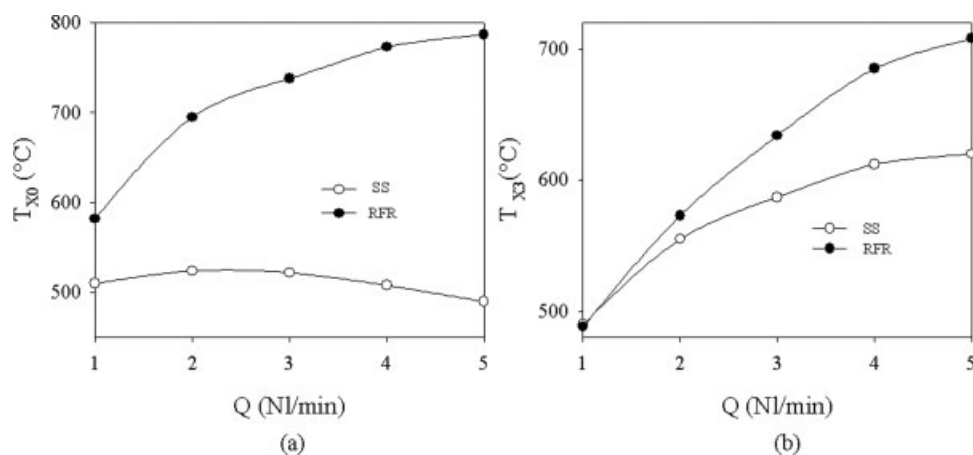
Figure 12. T_{X0} (a) and T_{X3} (b) as a function of total flow rate in steady state and reverse flow mode ( \tau = 350 s).
