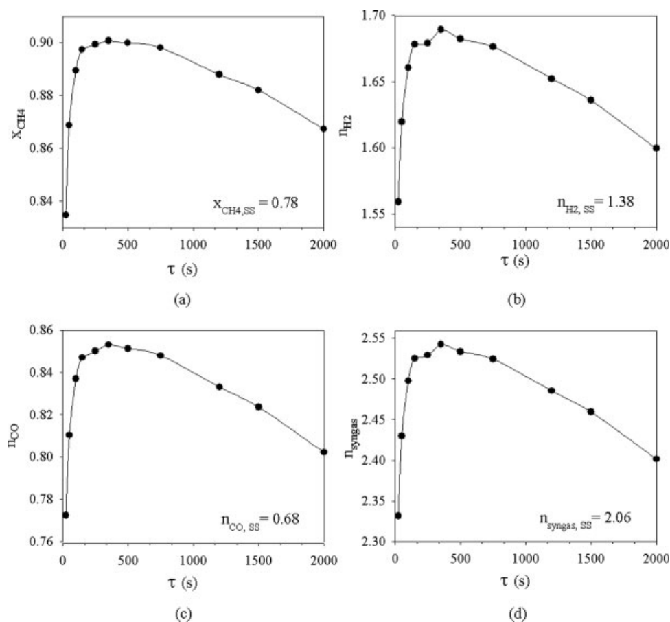
Figure 7. x_{\text{CH}_4} (a), n_{\text{H}_2} (b), n_{\text{CO}} (c), and n_{\text{syngas}} (d) as a function of \tau . Reaction conditions: \text{CH}_4/\text{O}_2 = 1.8 ; total flow rate Q = 4 NI/min.
