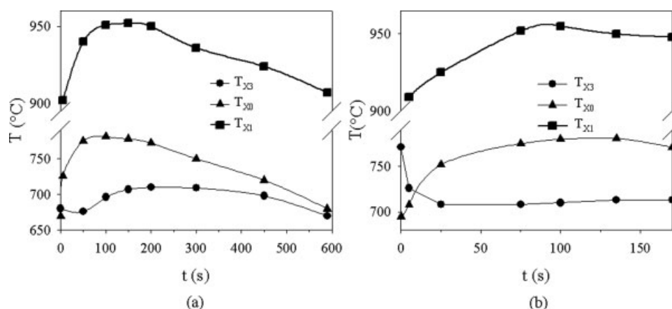
Figure 6. Temperature evolution at position x_0 , x_1 , and x_3 as a function of time: \tau = 1200 s (a); \tau = 350 s (b).
