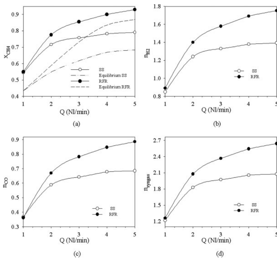
Figure 9. x_{CH_4} (a), n_{H_2} (b), n_{CO} (c), and n_{syngas} (d) as a function of total flow rate Q for stationary and reverse flow conditions ( \tau = 350 s).
