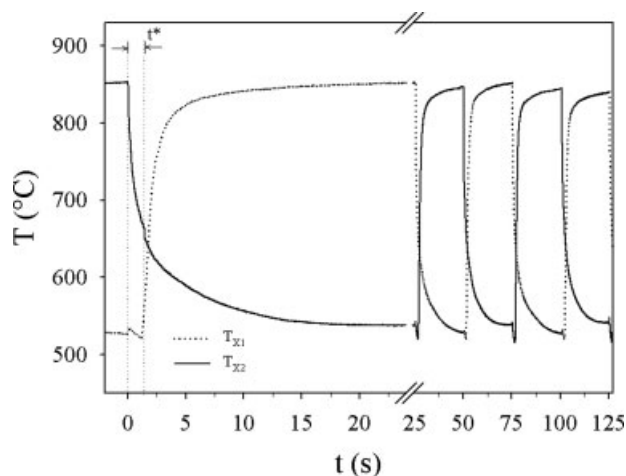
Figure 3. Temperature evolution in correspondence to x_1 and x_2 as a function of time.
